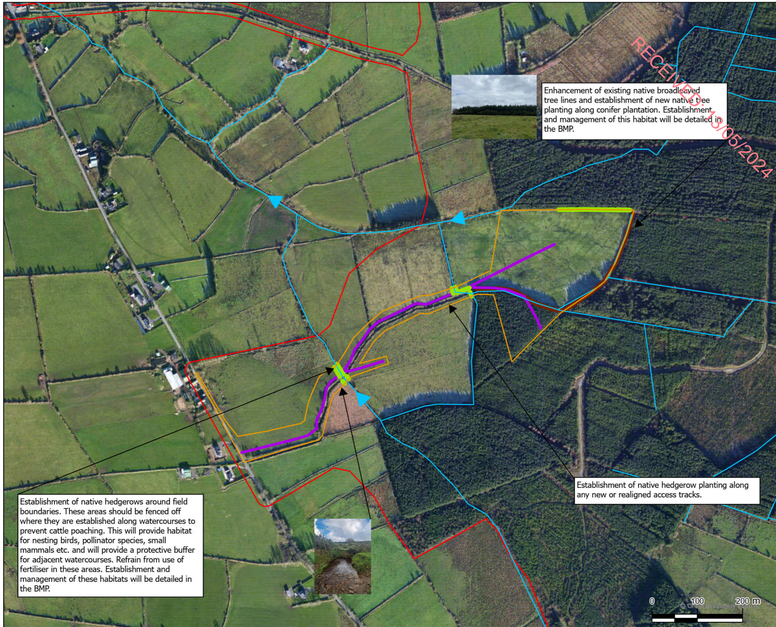
Figure 3-4 - Proposed Biodiversity Enhancement Options - Area 3
